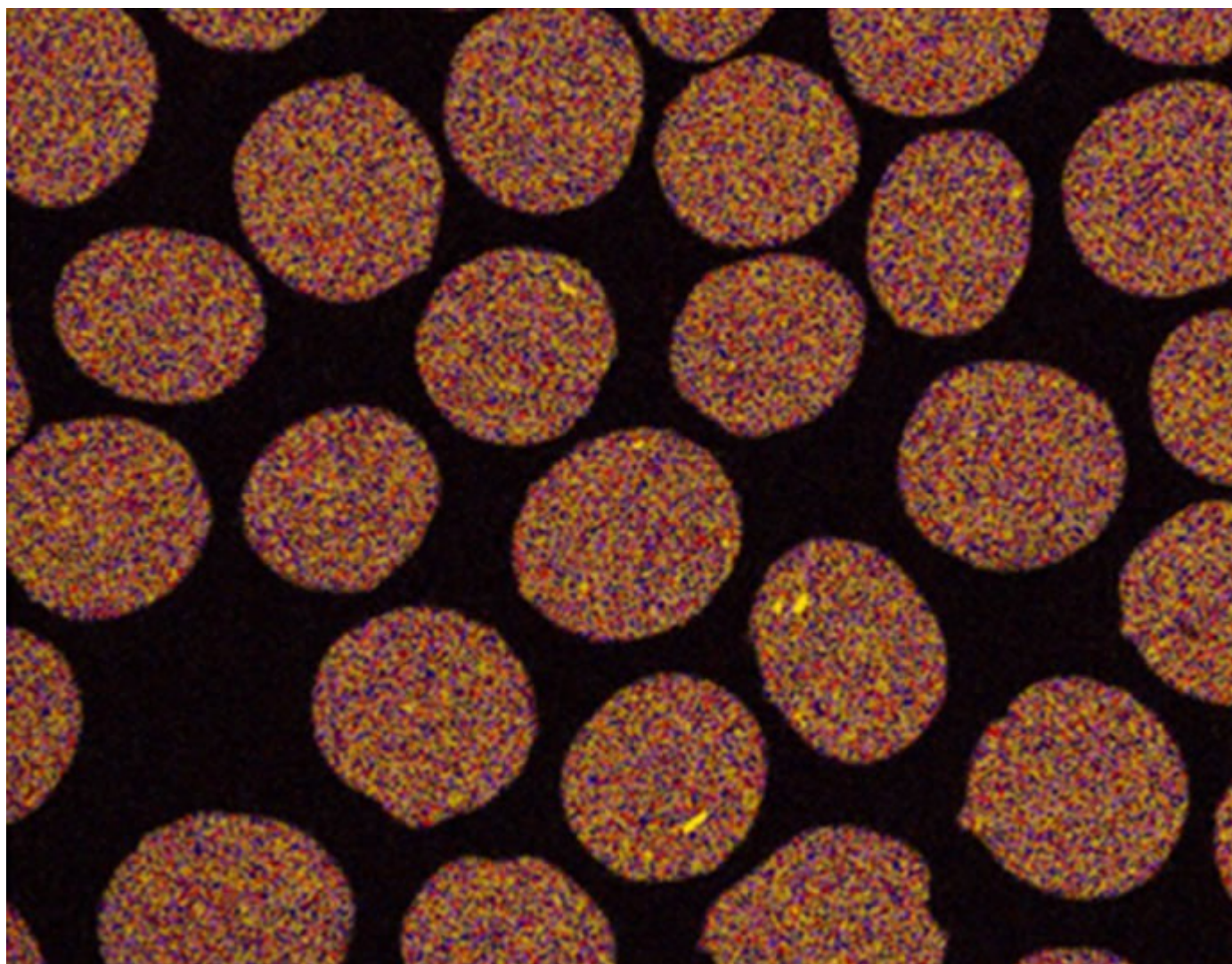
Overlay of minerals identified within a B-TRAXIM® All-in-① product. Each particle contains a combination of 4 different minerals
